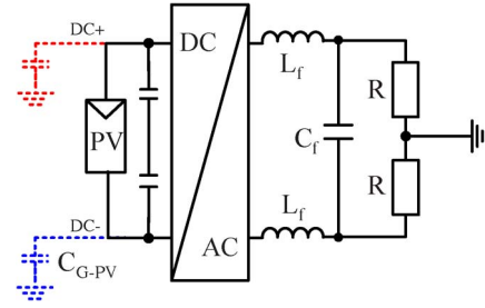
Fig. 2. Test setup used for common-mode voltage measurement.
