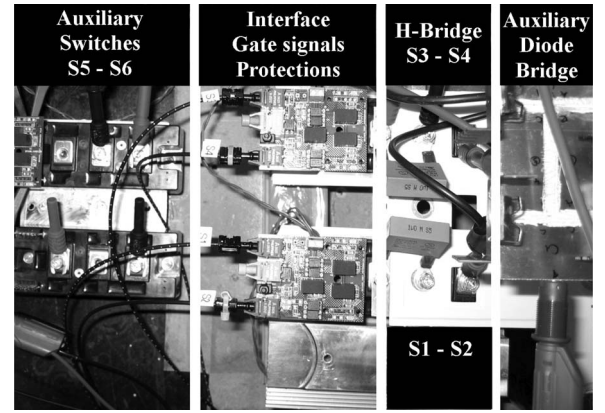
Fig. 16. Experimental setup: Modular solution.
