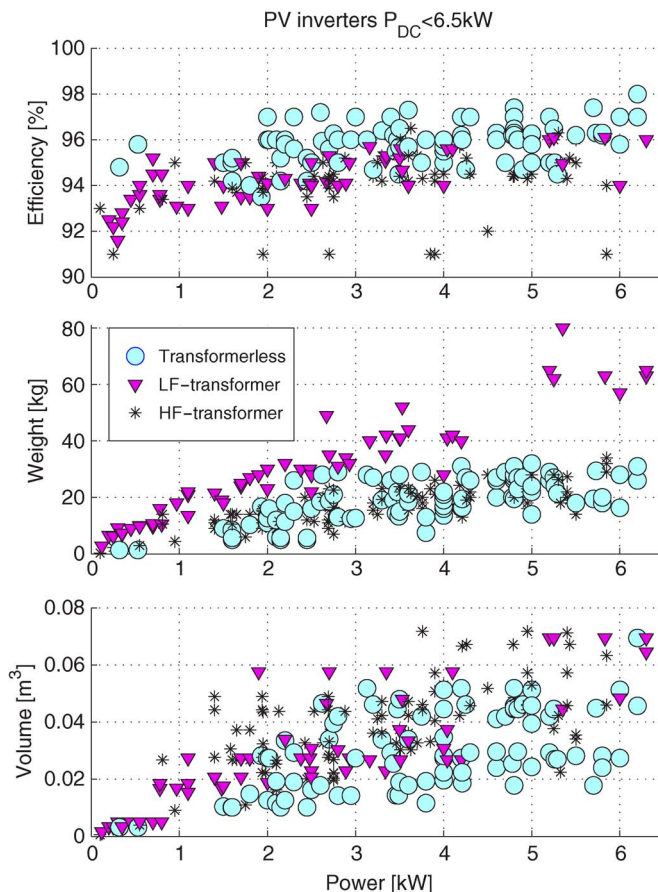
Fig. 1. Advantages and drawback of different inverter topologies.
